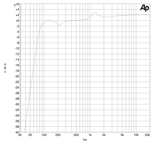
Amina LFiT EQ Response
