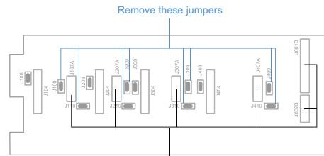
VTX-WMI card connectors
